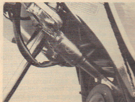
A slotted, knob-controlled device moves the steering damper pivot to give three settings.
